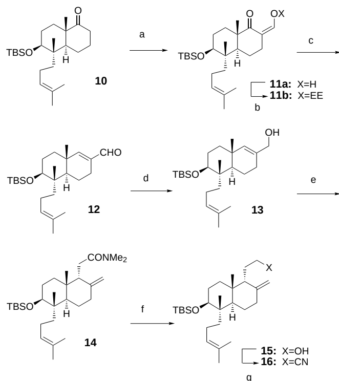
Scheme 3. Reagents and conditions: a) NaH/THF, ethyl formate, reflux; b) ethyl vinyl ether, \text{H}_3\text{PO}_4 (cat); c) 1. \text{NaBH}_4/\text{EtOH} ; 2. \text{HCl} (0.5 N), THF/water, 80% over four steps; d) \text{NaBH}_4/\text{EtOH} , 100%; e) N,N -dimethyl acetamide dimethyl acetal, m -xylene, reflux, 87%; f) superhydride, THF, 99%; g) 1. \text{MeSO}_2\text{Cl} , \text{Et}_3\text{N} , \text{CH}_2\text{Cl}_2 ; 2. \text{NaCN} , DMF, 100%. DMF = N,N -dimethylformamide.
