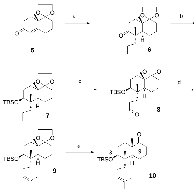
Scheme 2. Reagents and conditions: a) 1. Li/liquid ammonia/THF/ t BuOH, -78^{\circ}\text{C} \rightarrow \text{RT} ; 2. allyl bromide (6.25 equiv), 78%; b) 1. NaBH 4 /EtOH, -78^{\circ}\text{C} \rightarrow \text{RT} ; 2. TBSOTf, 2,6-lutidine, CH 2 Cl 2 , -78^{\circ}\text{C} \rightarrow \text{RT} , 83%; c) 1. BH 3 ·THF, room temperature; 2. NaOH/H 2 O 2 , reflux; 3. PCC, CH 2 Cl 2 , 56%; d) isopropyltriphenylphosphonium iodide, t BuLi, DMSO, 85%; e) PPTS, acetone, reflux, 96%. TBSOTf = tert -butyldimethylsilyl trifluoromethanesulfonate; PCC = pyridinium chlorochromate; DMSO = dimethyl sulfoxide; PPTS = pyridinium p -toluenesulfonate.
